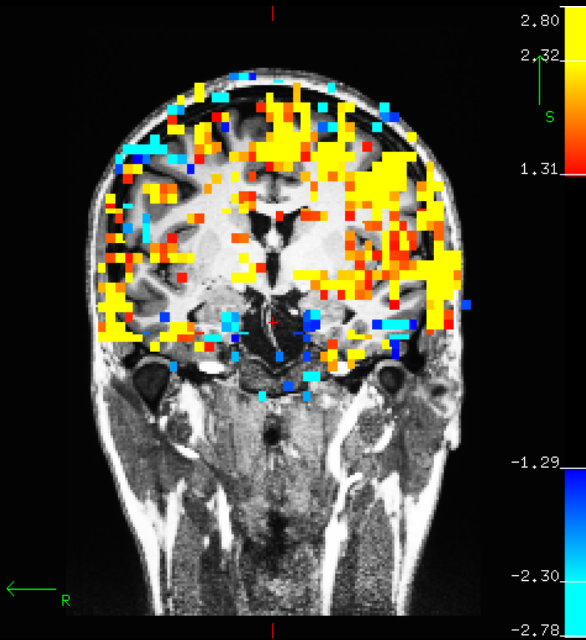
Native Space
