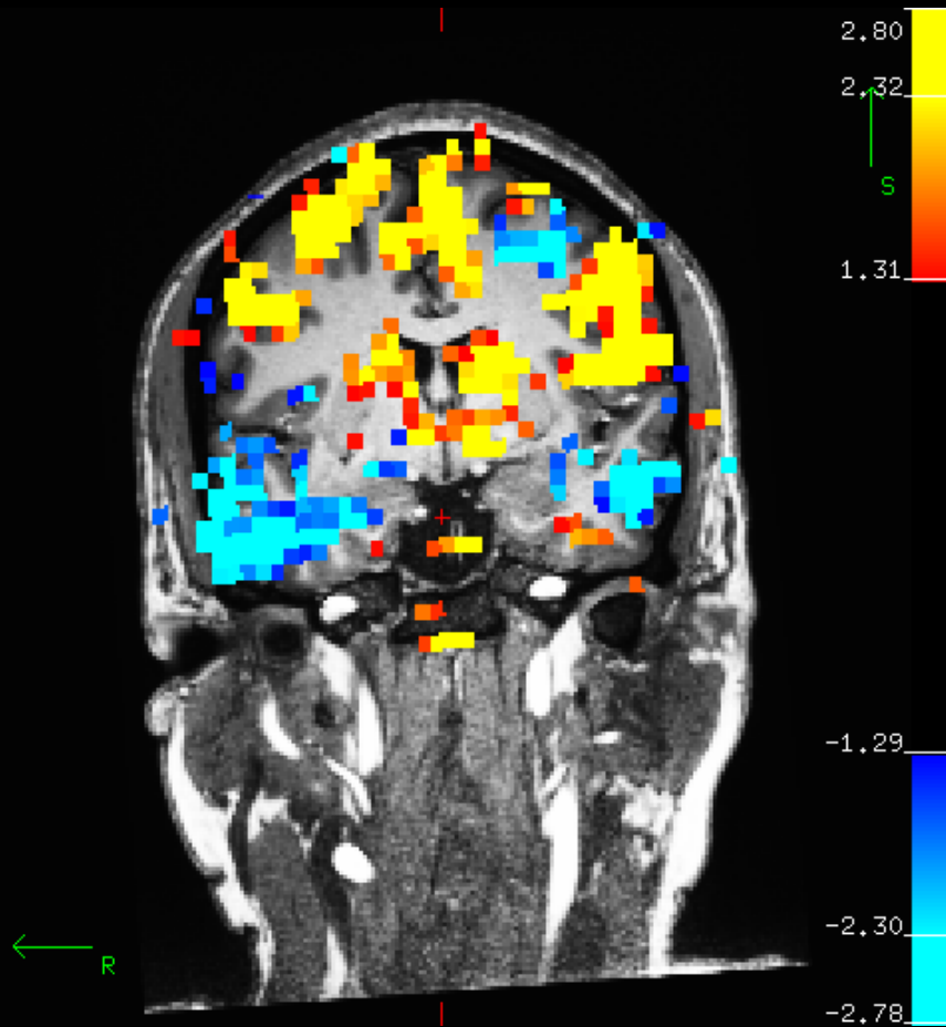
Native Space
